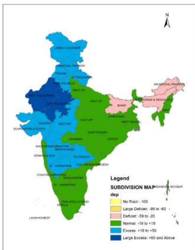
Fig. 1: Seasonal rainfall status (01 June – 30 September 2025) in 36 meteorological subdivisions, India
